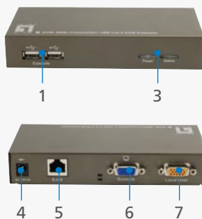
KVM-9006(Transmitter)
