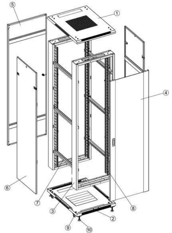
1. Top cover, 2. Bottom panel, 3. Door frame, 4. Front door 5. Rear door, 6. Side panel, 7. Horizontal beam, 8. Vertical Rail, 9. Caster (2 with brake), 10. Levelling feet
